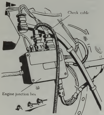
FIGURE 10-73. Check cable connected to engine junction box.
